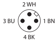
Fig. 11: pin layout
