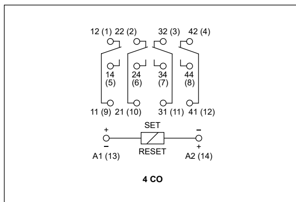
Connection diagram (pin side view)
