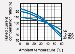
Temperature curve
