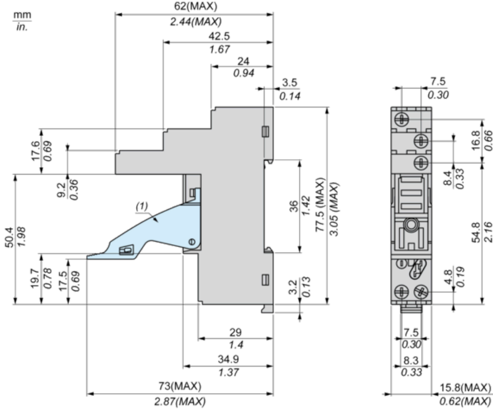
(1) Maintaining clamp
