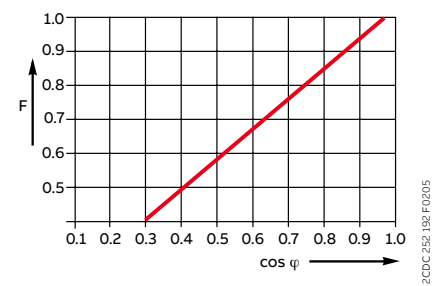
Derating factor F for inductive AC load
