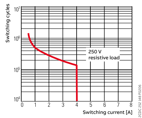
Contact lifetime
