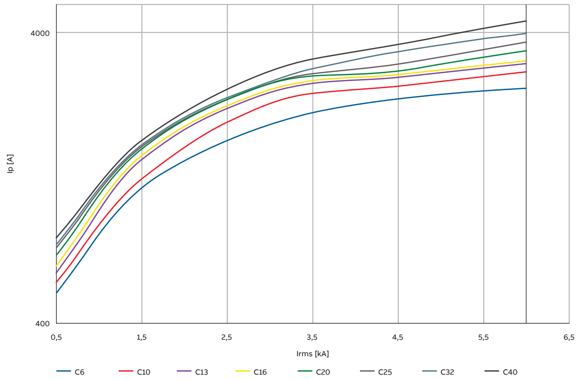
I peak DSH201 - Characteristic C
