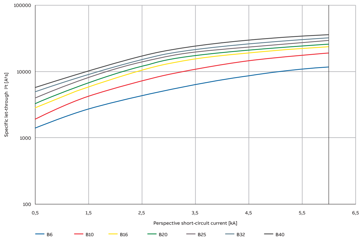
Specific let-through energy I^2t DSH201 - Characteristic B
