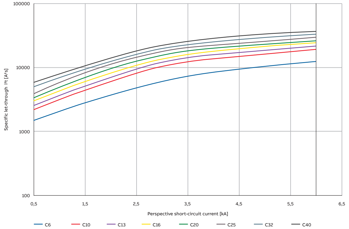
Specific let-through energy I^2t DSH201 - Characteristic C
