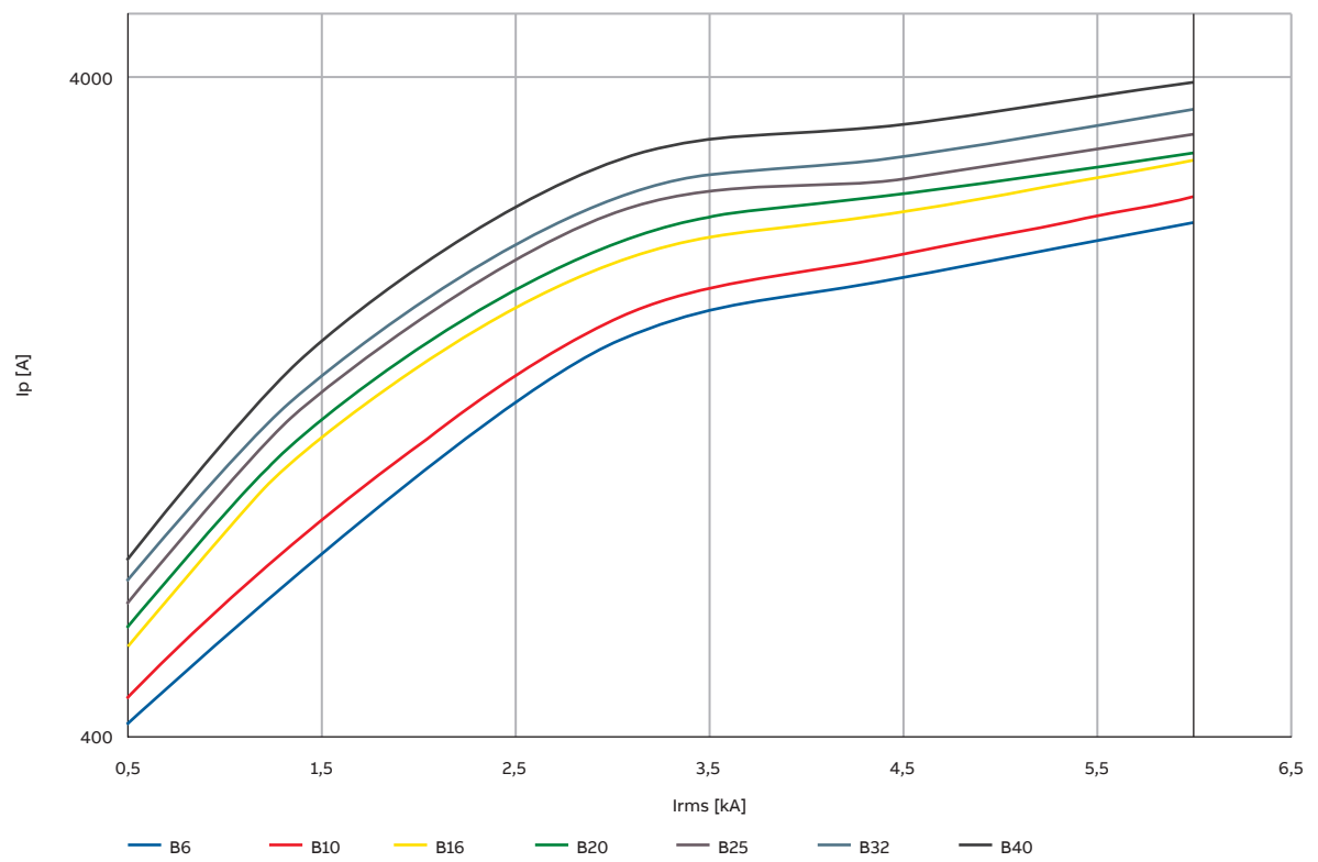
I peak DSH201 - Characteristic B
