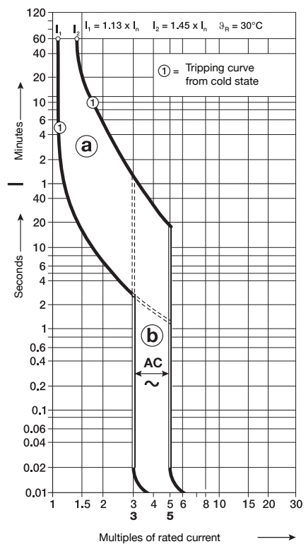
Tripping characteristics B IEC/EN 61009-1
