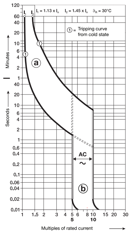
Tripping characteristics C IEC/EN 61009-1
