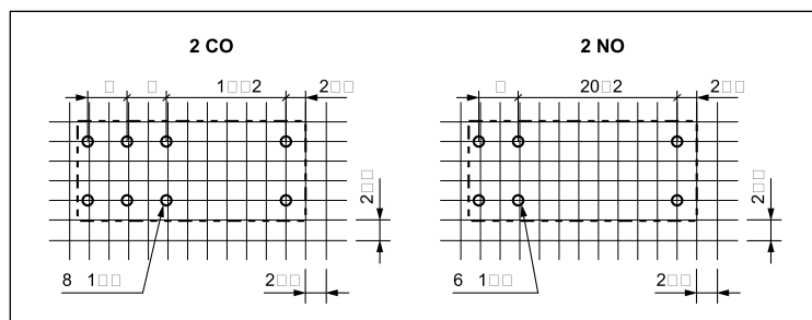
Pinout (solder side view)
